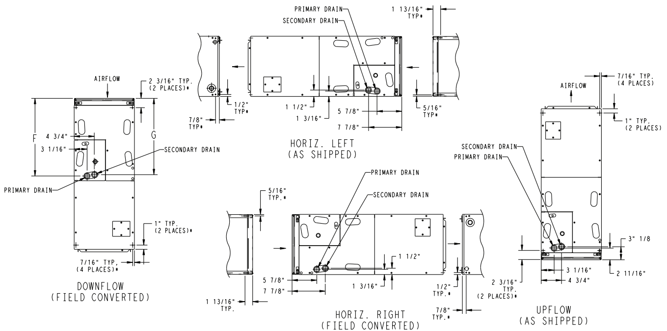
Fig. 2 – PF4MNB – English
